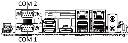
Serial Port connector
