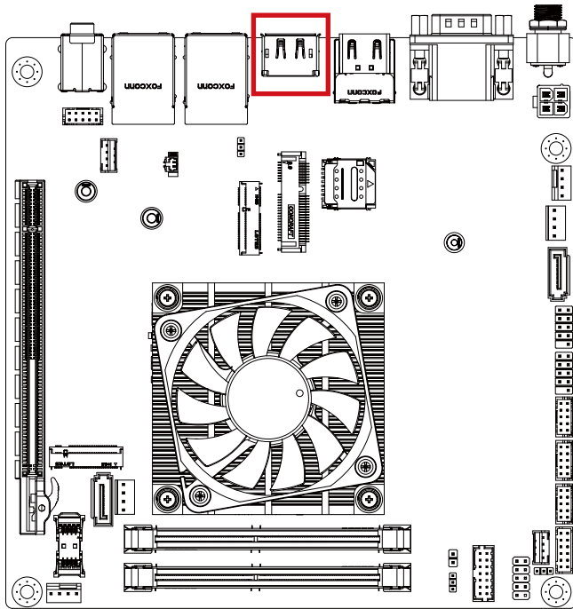
DP connector
