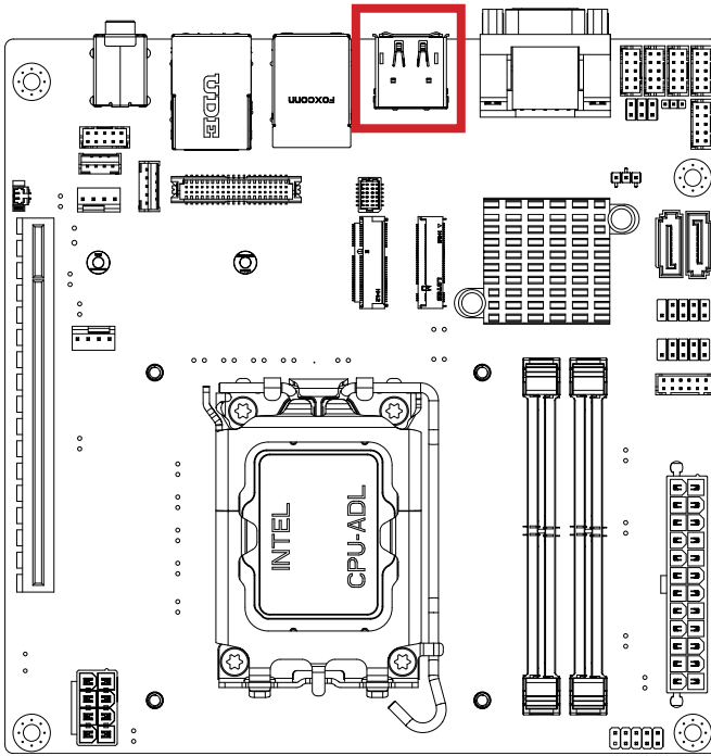
HDMI & DP Connector
