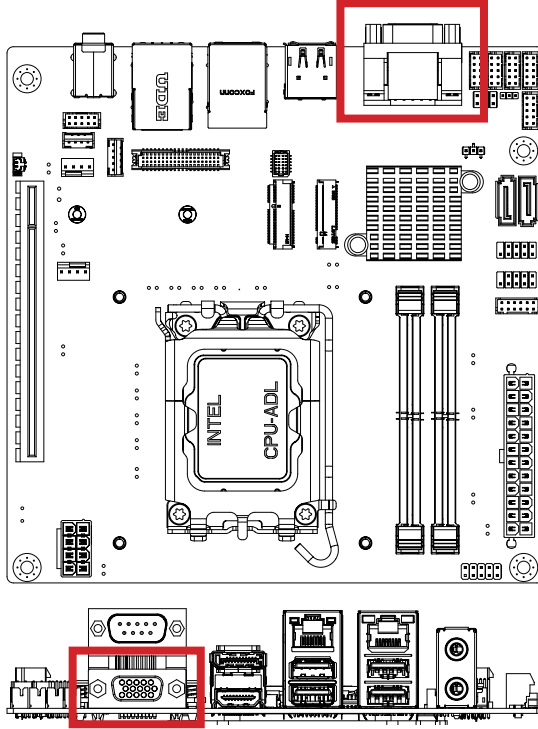
D-sub Connector
