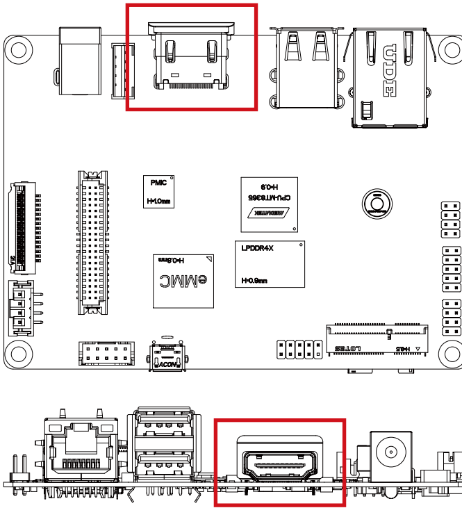
HDMI Connector
