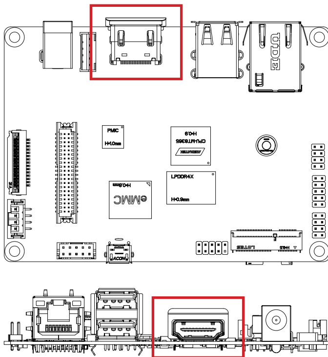
HDMI Connector
