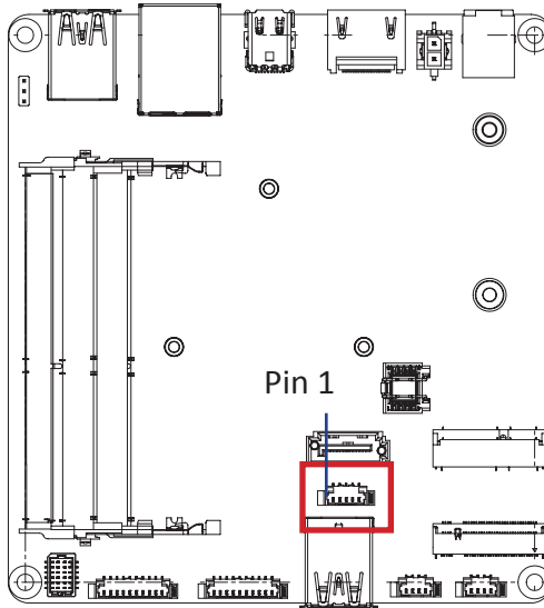
SATA 6Gb/s power connector
