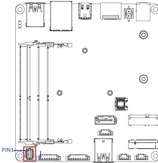
Front Panel Connector
