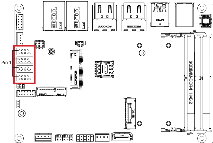
Serial Port Connector
