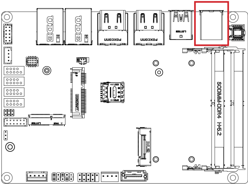
USB 2.0 connector
