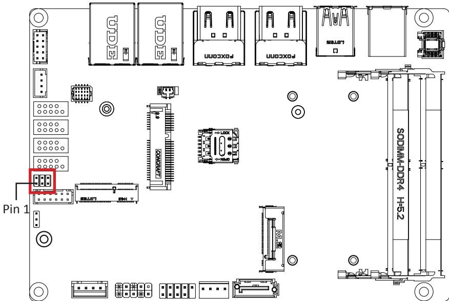
JCOM Jumper Select
