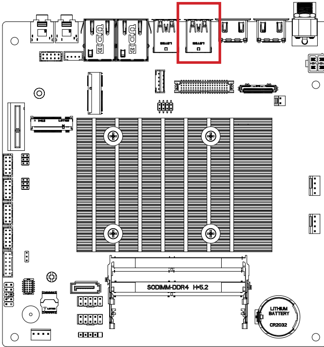
USB Connector
