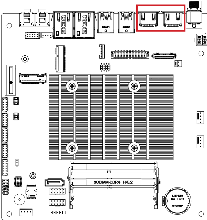
HDMI connector
