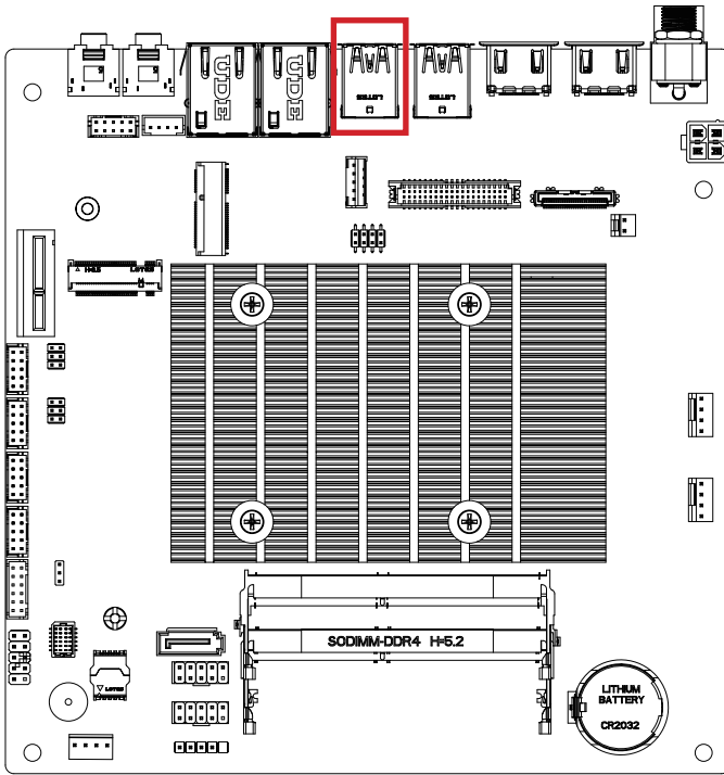
USB connector
