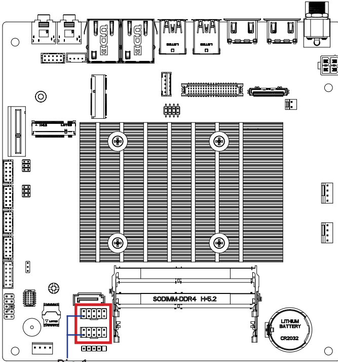
Pin 1
