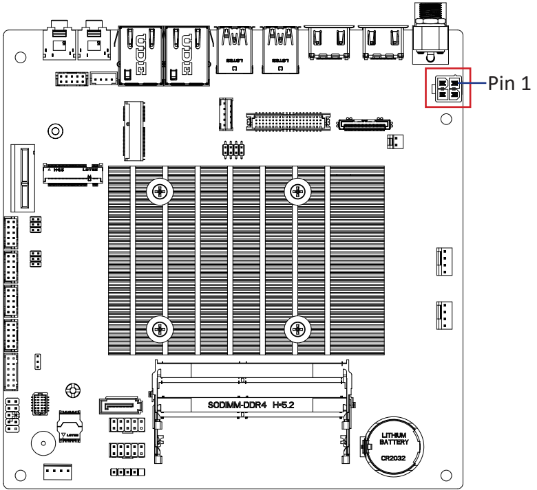
Power Connector
