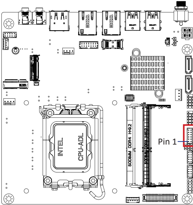
GPIO Connector
