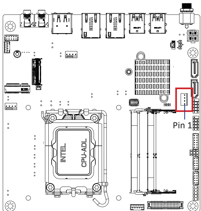
SATA Power Connector
