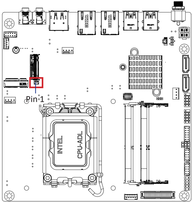
Buzzer header
