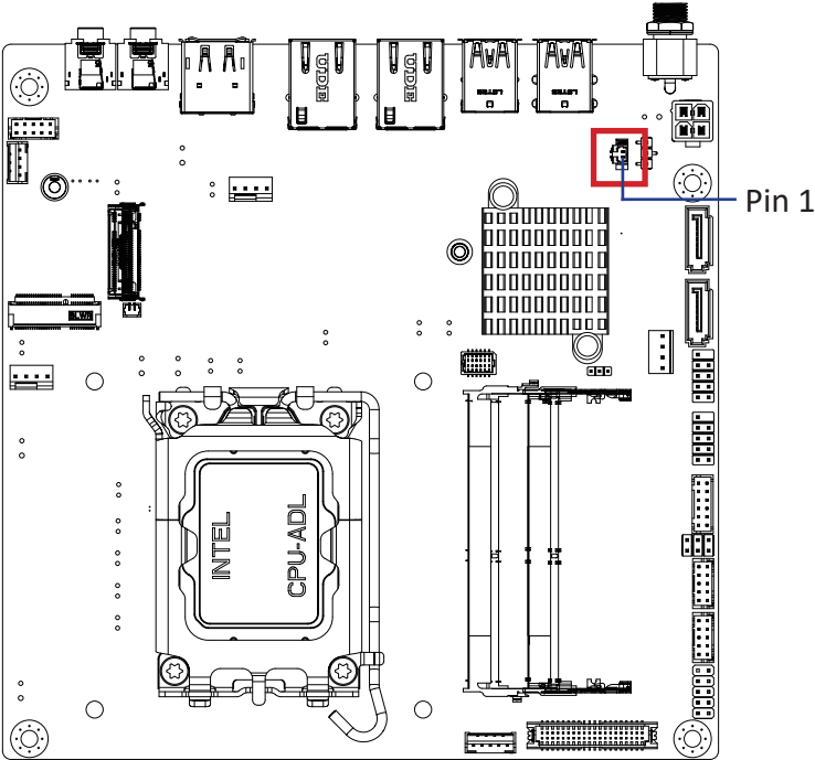
Battery Connector
