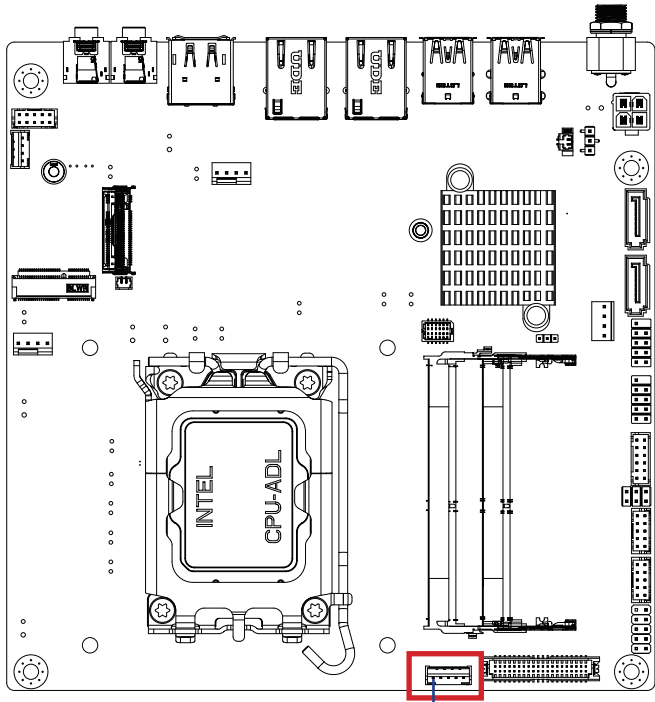
Backlight Control header
