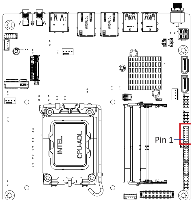
GPIO Connector
