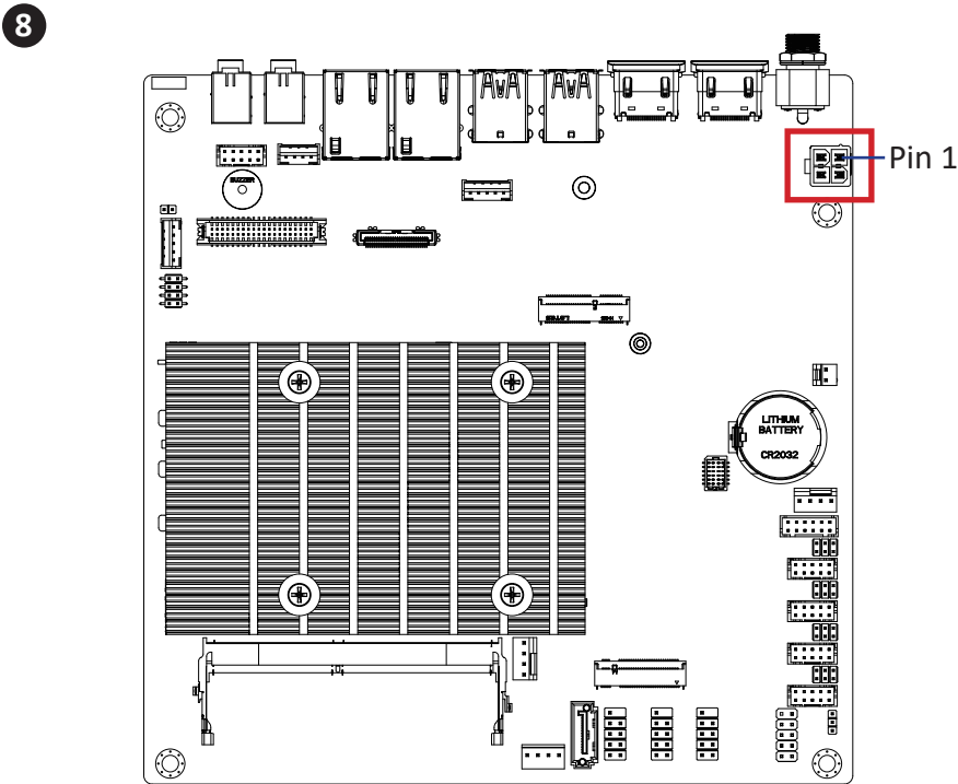
power Connector
