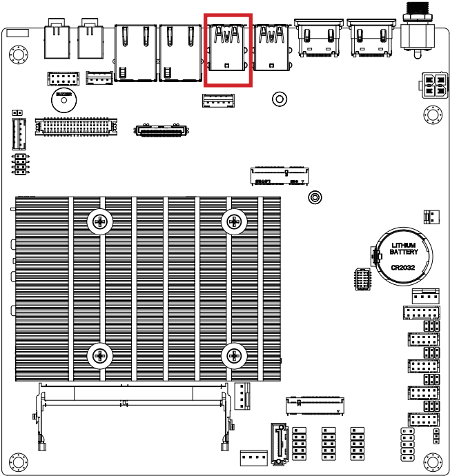
USB 3.2 Gen 1 connector
