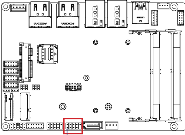
USB 2.0 Header
