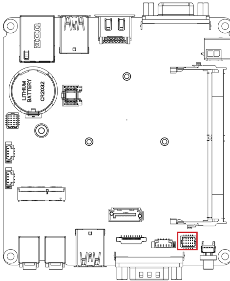
F_PANEL (Front Panel Header)
