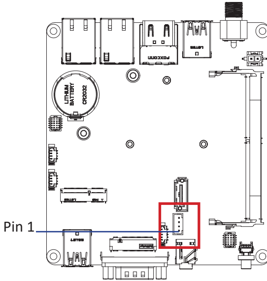
Speaker Out connector
